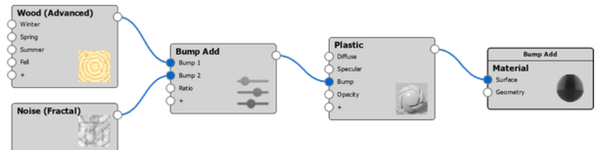
The Material Graph structure of this example
