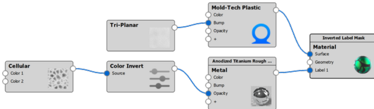
The Material Graph structure of this example.
