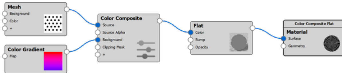
The Material Graph structure of above composite
