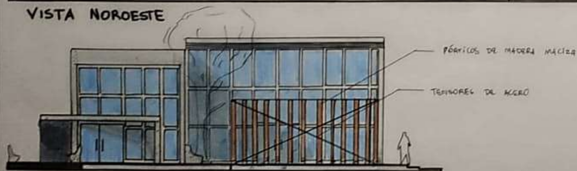
VISTA FRONTAL
